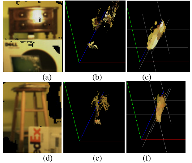
Figure 2: Occluded Landmark left image of stereo pair (a,d), perspective view of image pixels mapped to absolute depth (b,e), perspective view of terrain spatiogram showing XZ clusters (c,f)
