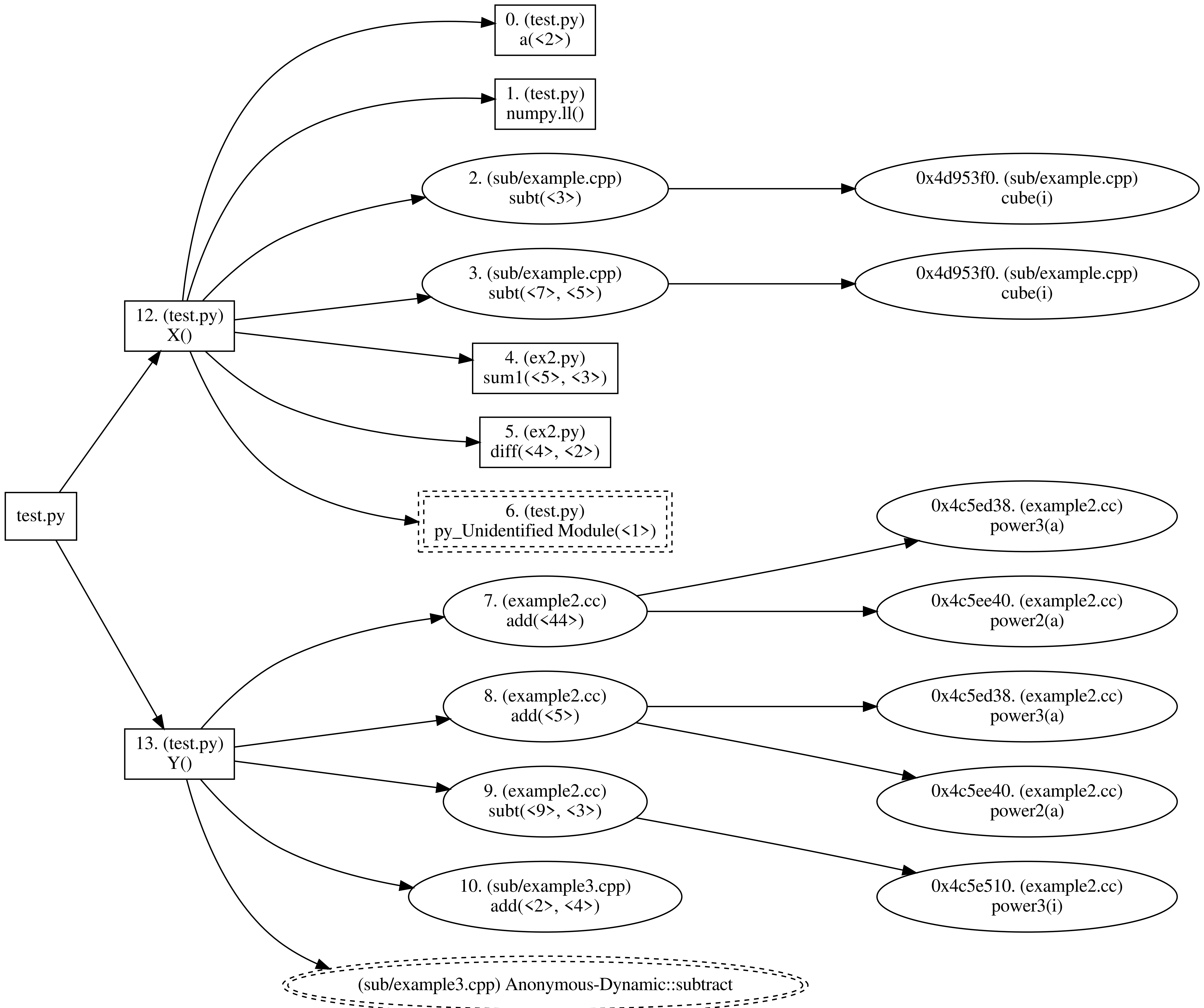
test Call Graph
